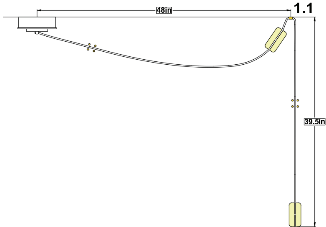
SNAPS LARGE LED PENDANT · 401850 WITH 905701 24" STRAP WITH LED Configuration 1 · 39.5" h x 48" w
