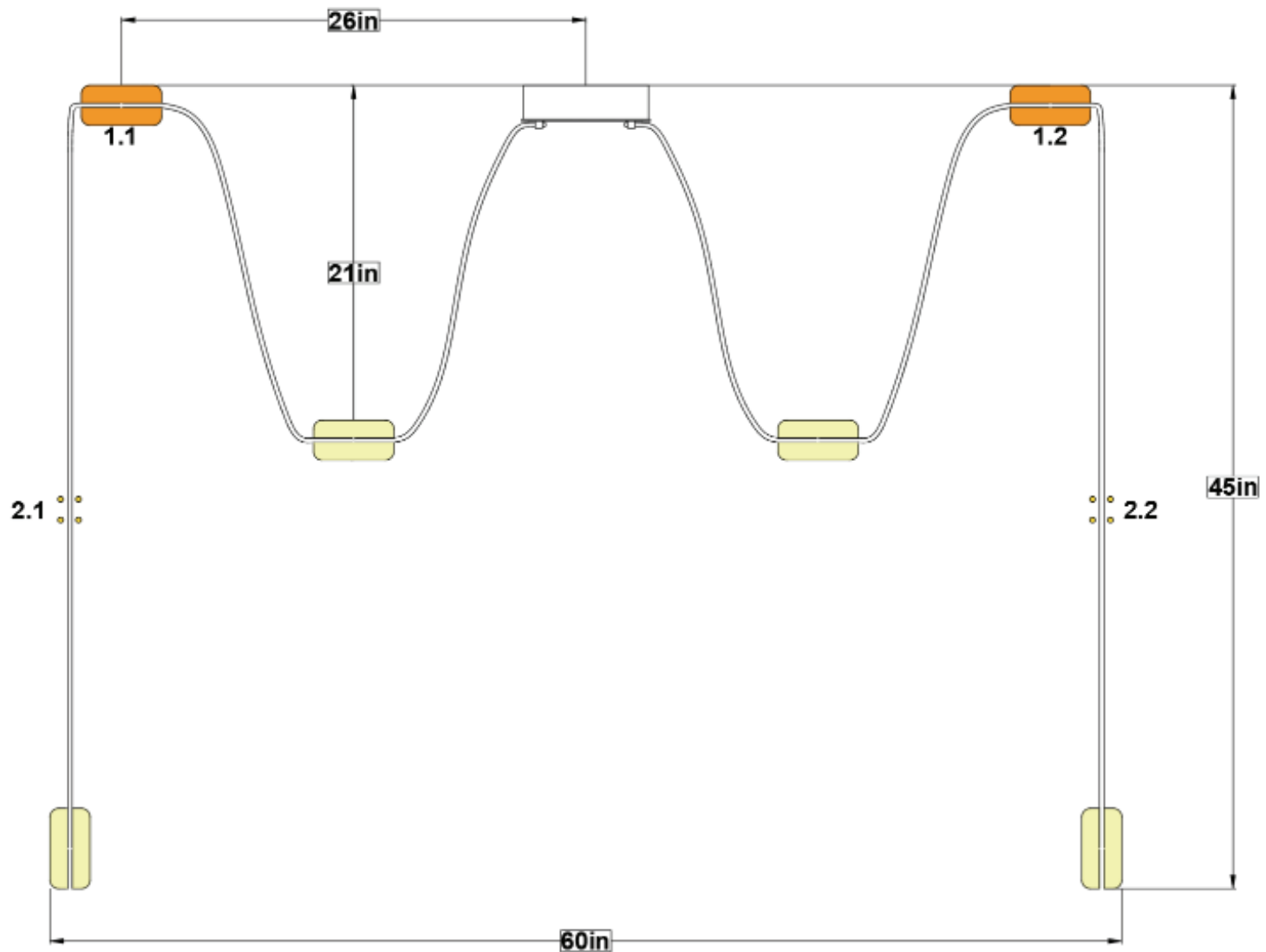
SNAPS MEDIUM LED PENDANT · 401315 Configuration 1 · 45" h x 60" w x 4" d
